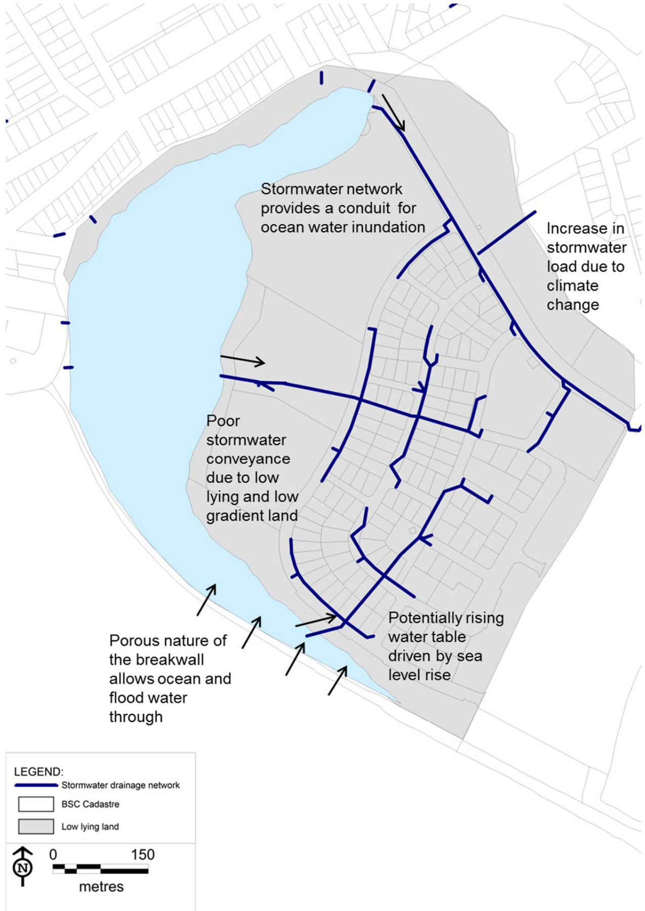
Figure 6: Inundation process
