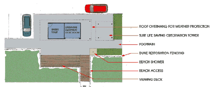
ENLARGED PLAN SECTION 1:200 @ A1
