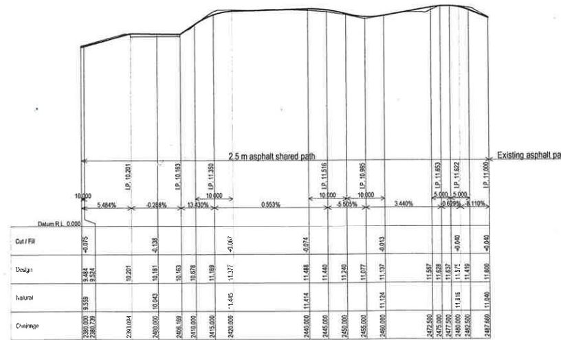
Longitudinal Section Horizontal Scale A, Vertical Scale B
