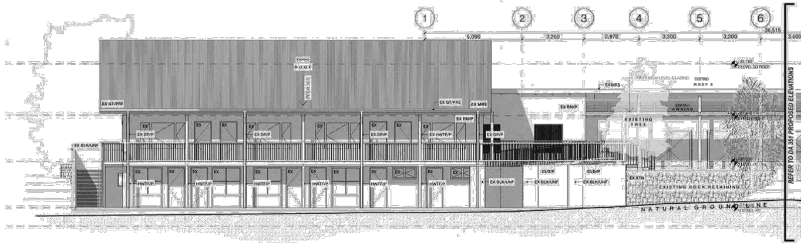
01 PROPOSED EAST ELEVATION
