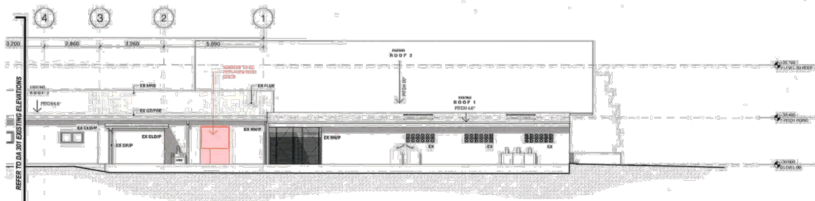
04 EXISTING WEST ELEVATION EX 04/01/01
