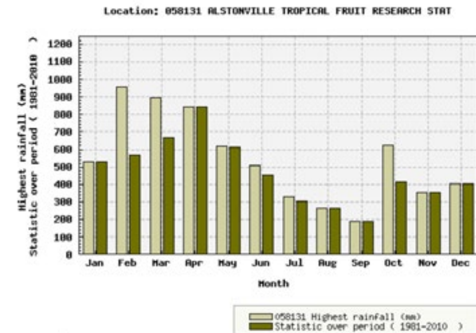
Diagram 4: 1981 – 2010 Rainfall Data – Alstonville Tropical Fruit Research Station
