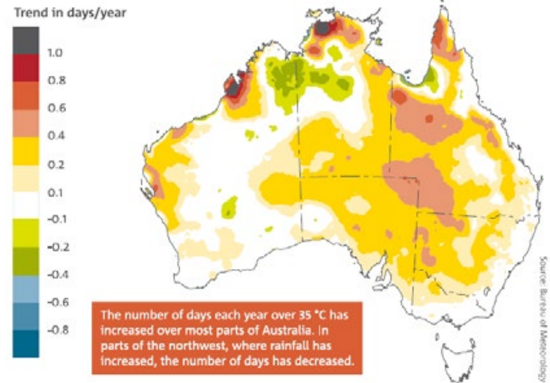
Diagram 48: Trend in days per year above 35°C
