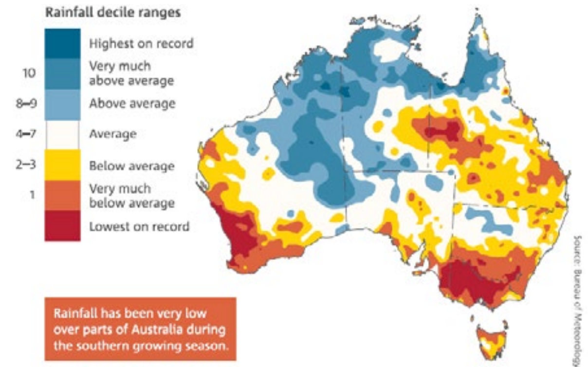
Diagram 49: Rainfall decile ranges 1996 - 2015
