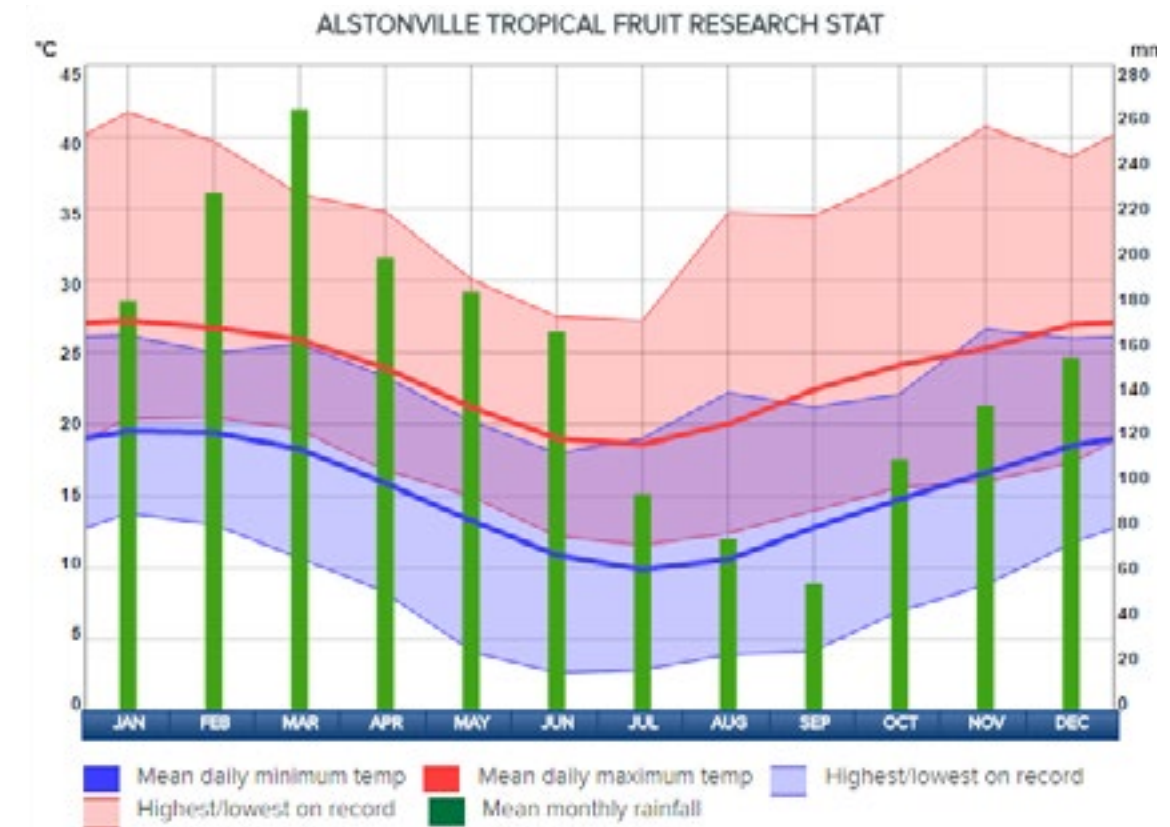
Diagram 3: Alstonville Annual Temperature and Rainfall Data
