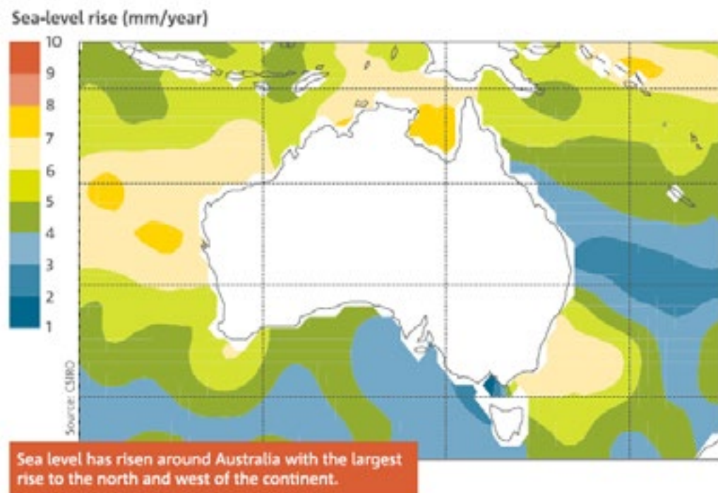
Diagram 47: Annual sea level rise estimates
