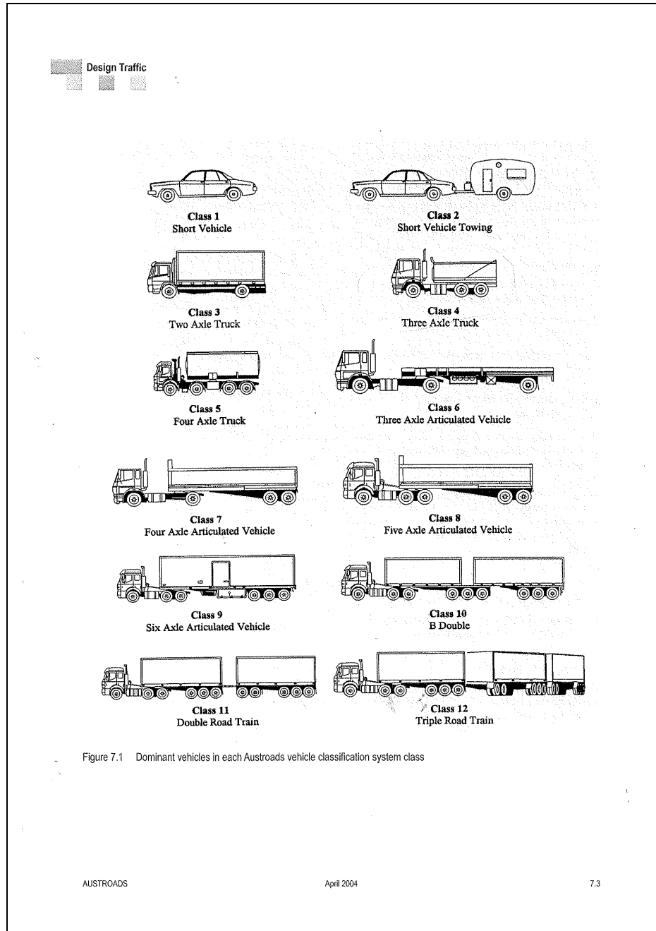
Figure 1: Austroads 2004 Vehicle Classifications
