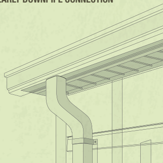
Temporary or permanent downpipe
