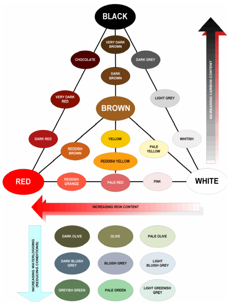
Figure 3. Colour triangle showing relationships between soil colours and influencing factors/conditions
